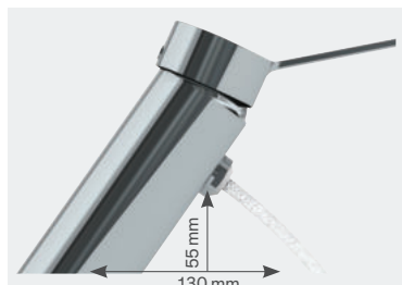
JET 2621MINIEP Ref. DELABIE - 2621MINIEP_jet
